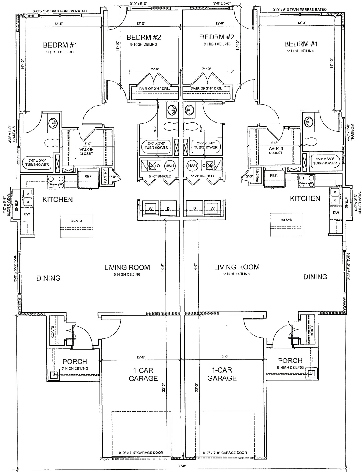
Transitional Housing – Duplex Floor Plan
